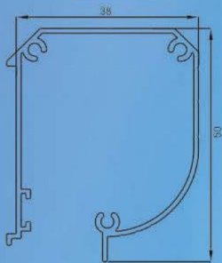
Store Roller
