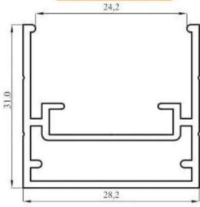
N1 Side Profile (Side-Bottom Profile)
