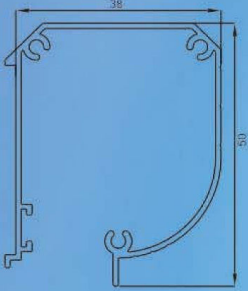
Store Roller
